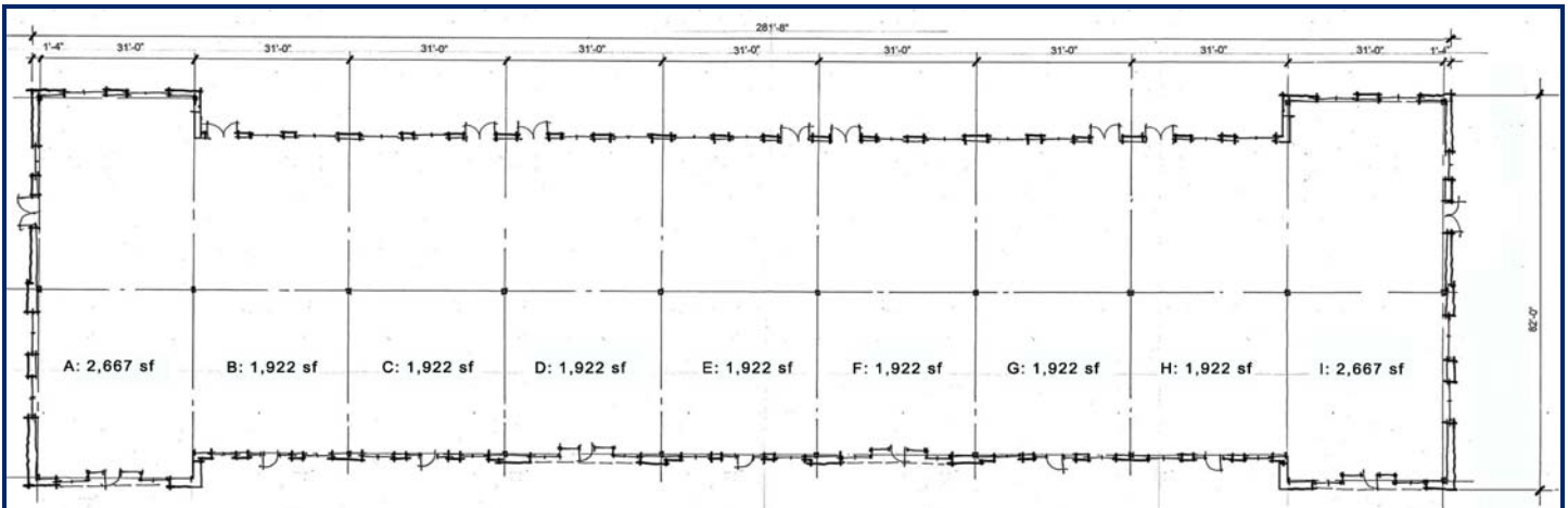
Floor Plan
