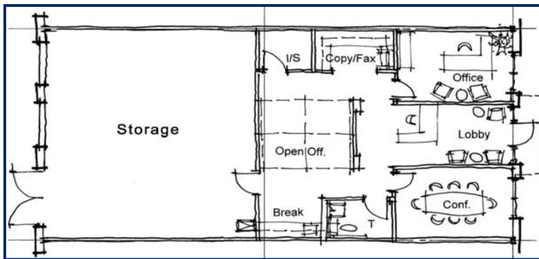
Sample Office & Warehouse Plan
